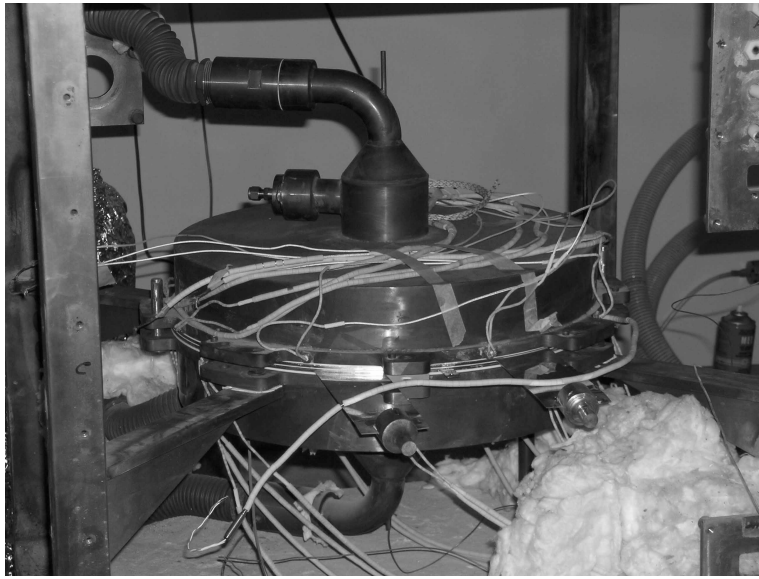
Figure 1 – The experimental cylindrical MCFC
